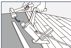
Nail-Down Installation
